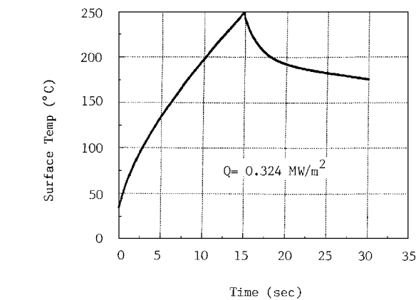
Fig. 9b Steady-state response of the surface temperature during the combined heating and cooling period.
