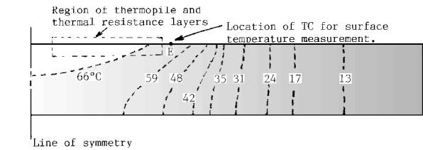
Fig. 11a Temperature profile in the entire heat flux gauge when t = 1.0 s and Q = 0.324 MW/m 2 ; temperature units: °C.
