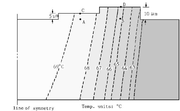
Fig. 11b Enlarged view of the temperature profile near thermopile tip locations A and B, time t = 1.0 s, and Q = 0.324 MW/m 2 ; geometry: not to scale.
